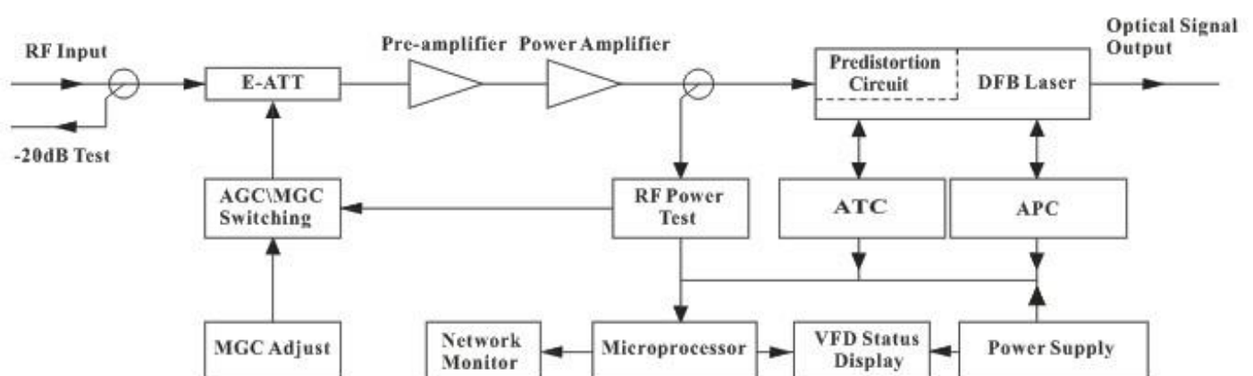
1550nm Direct Mode Optical Transmitter Block Diagram
